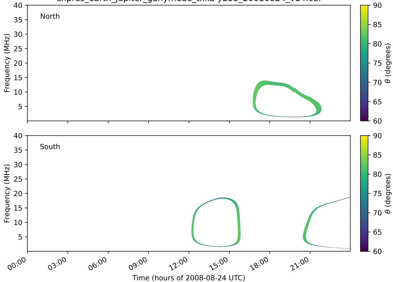
expres_earth_jupiter_ganymede_txka-y235_20080824_v14.cdf
