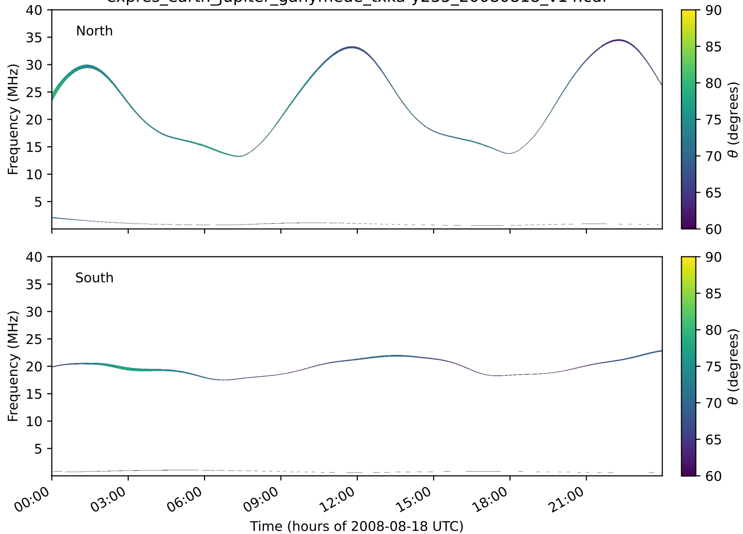
expres_earth_jupiter_ganymede_txka-y235_20080818_v14.cdf
