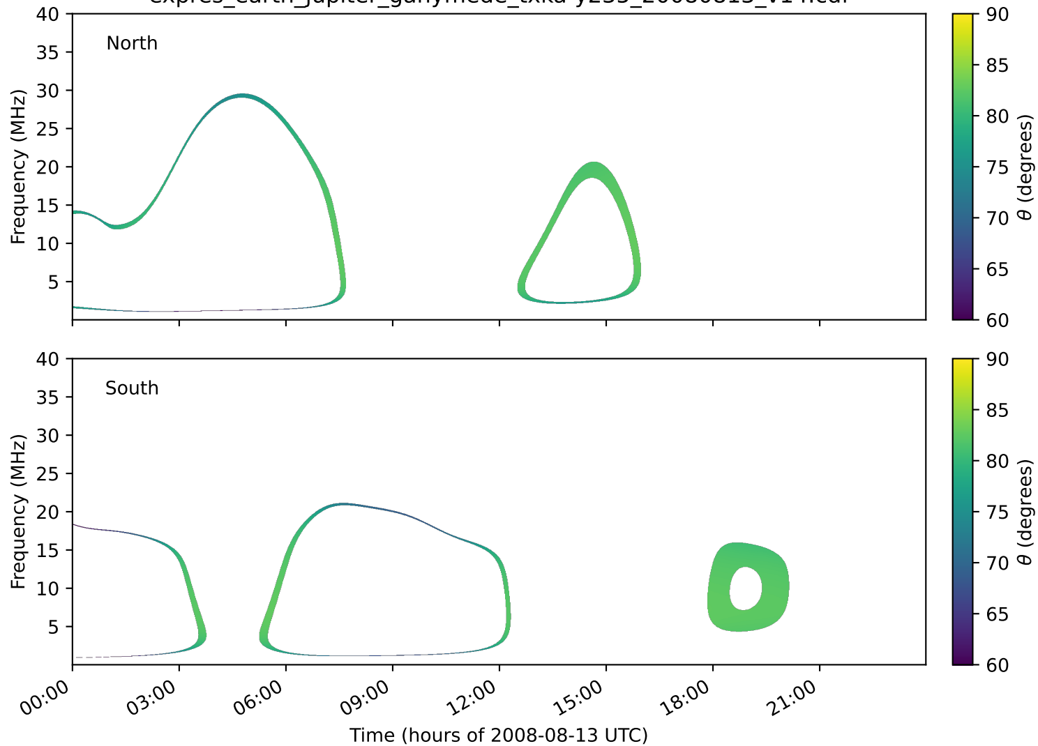
expres_earth_jupiter_ganymede_txka-y235_20080813_v14.cdf
