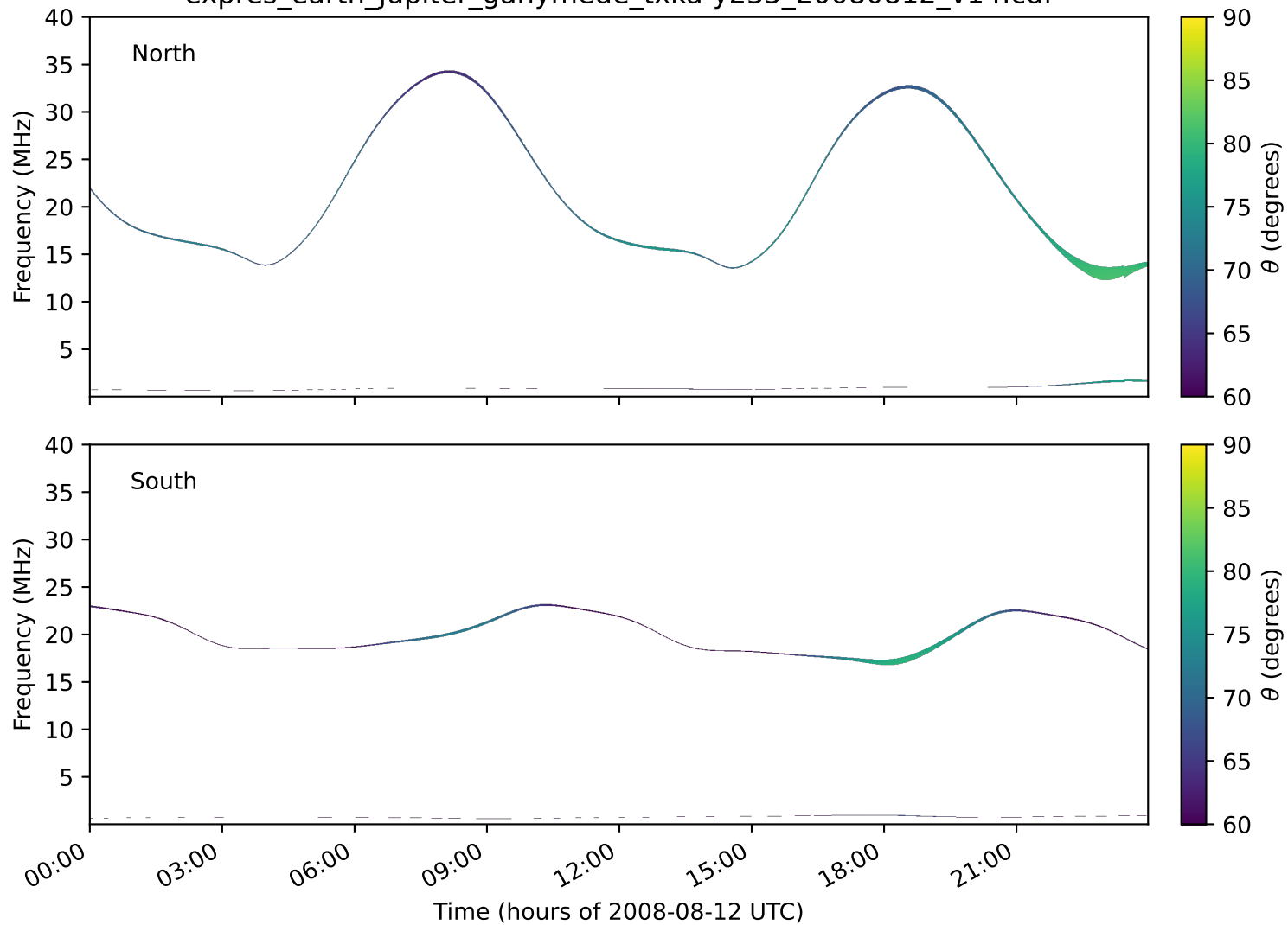
expres_earth_jupiter_ganymede_txka-y235_20080812_v14.cdf
