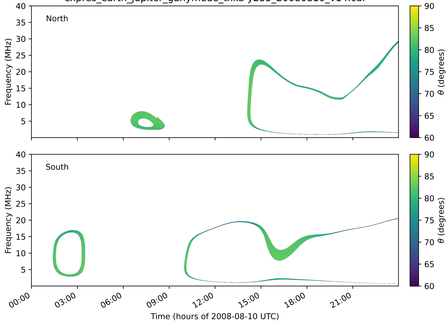
expres_earth_jupiter_ganymede_txka-y235_20080810_v14.cdf
