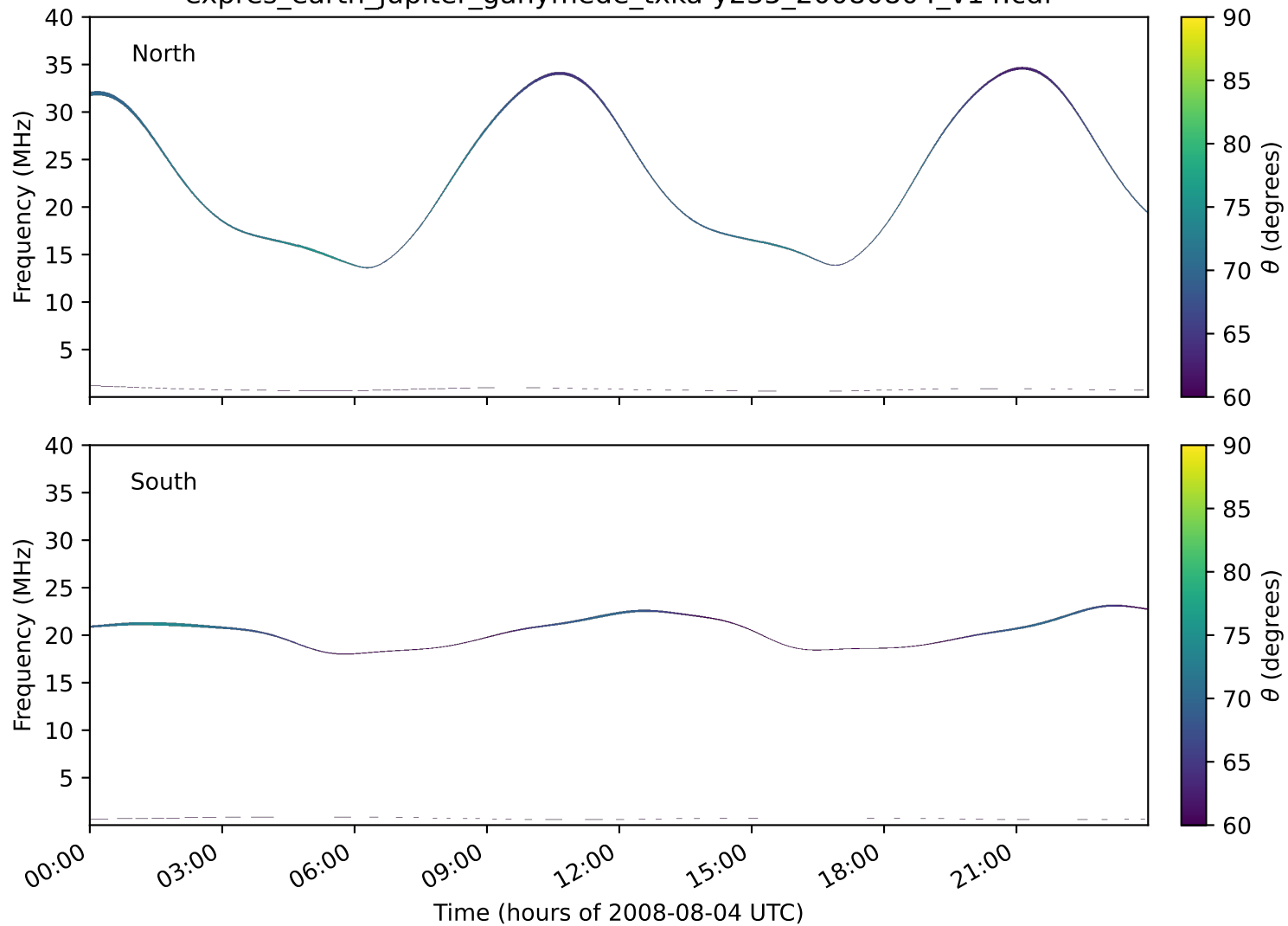
expres_earth_jupiter_ganymede_txka-y235_20080804_v14.cdf
