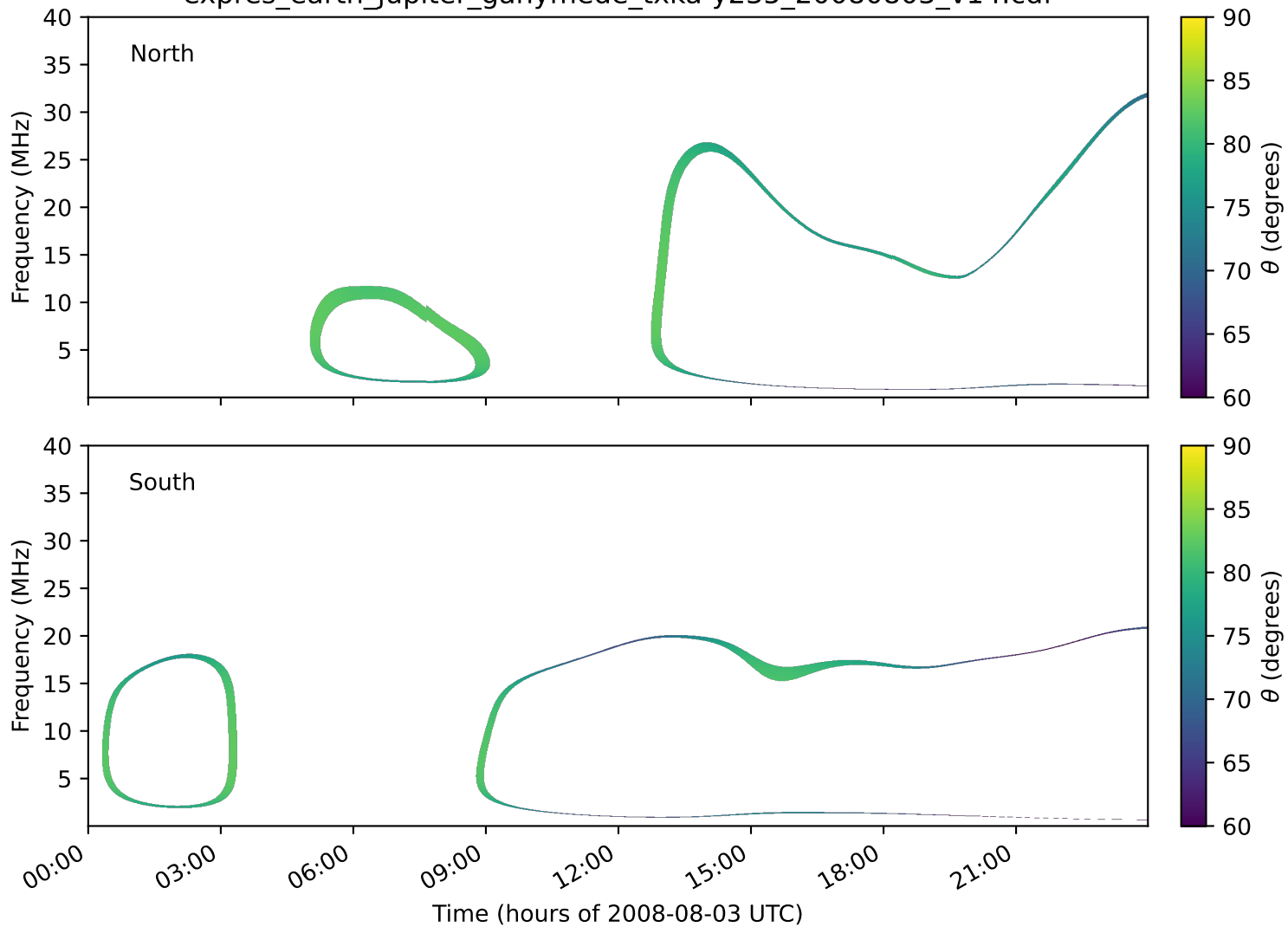
expres_earth_jupiter_ganymede_txka-y235_20080803_v14.cdf
