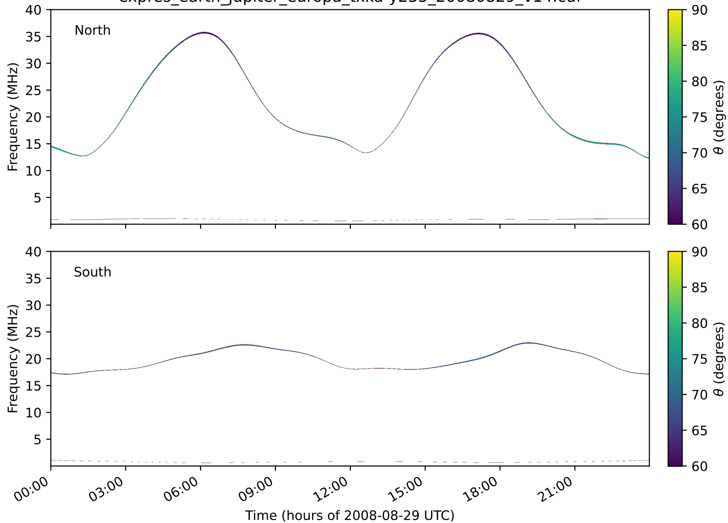
expres_earth_jupiter_europa_txka-y235_20080829_v14.cdf
