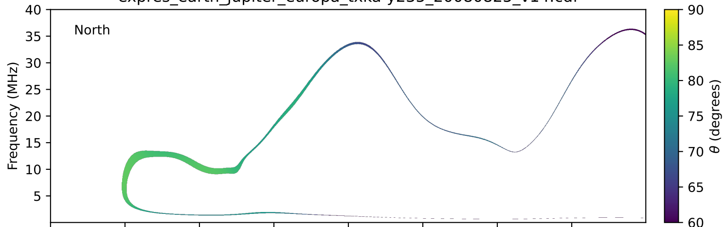
expres_earth_jupiter_europa_txka-y235_20080825_v14.cdf
