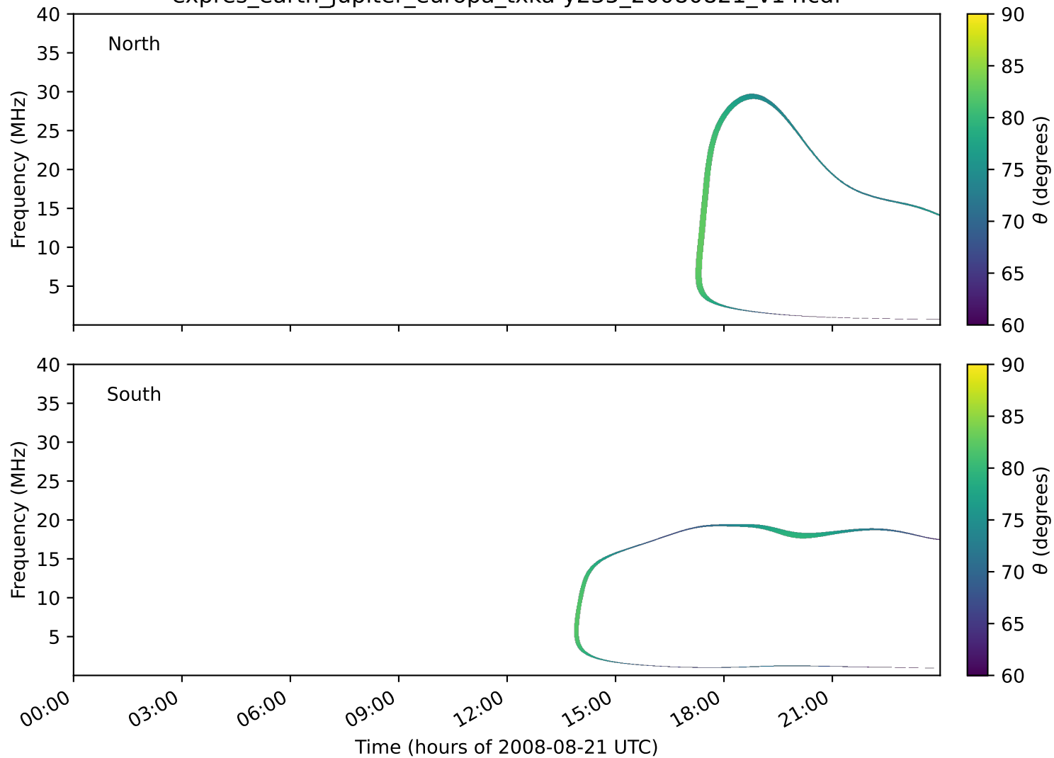
expres_earth_jupiter_europa_txka-y235_20080821_v14.cdf
