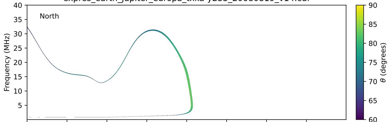
expres_earth_jupiter_europa_txka-y235_20080819_v14.cdf
