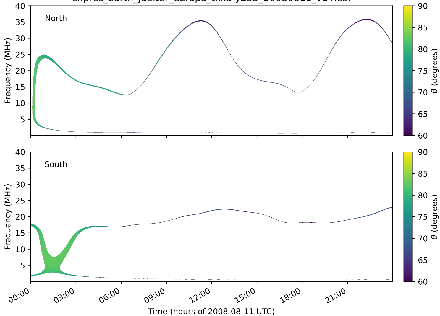
expres_earth_jupiter_europa_txka-y235_20080811_v14.cdf
