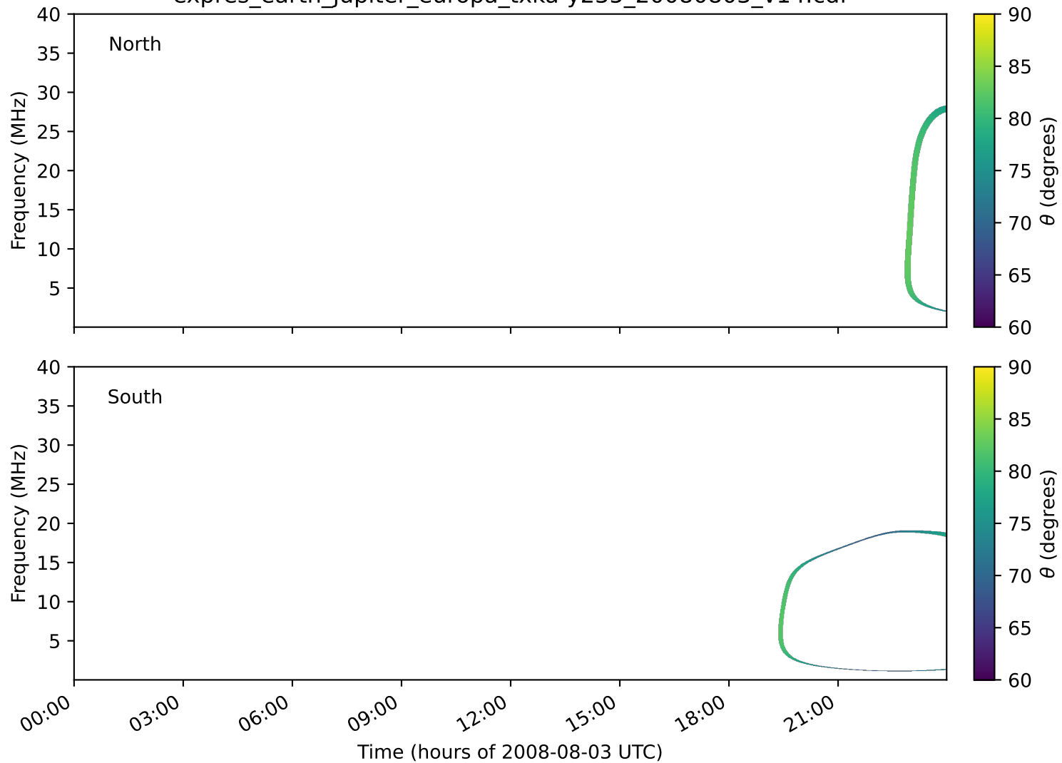
expres_earth_jupiter_europa_txka-y235_20080803_v14.cdf
