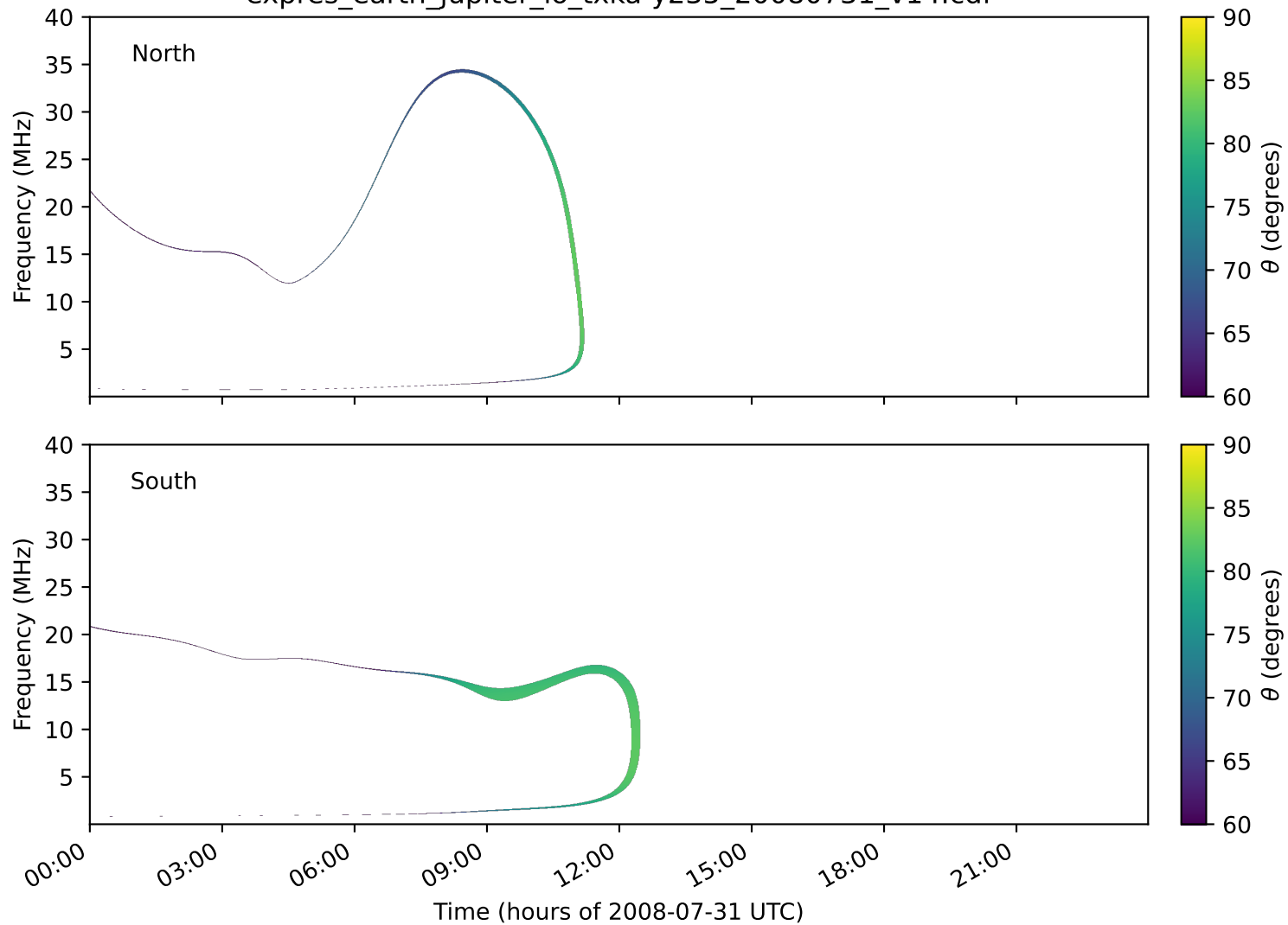
expres_earth_jupiter_io_txka-y235_20080731_v14.cdf
