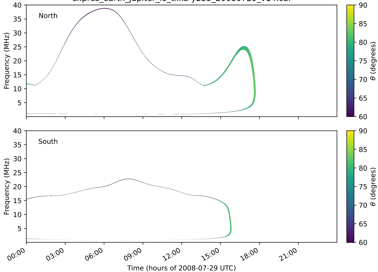
expres_earth_jupiter_io_txka-y235_20080729_v14.cdf
