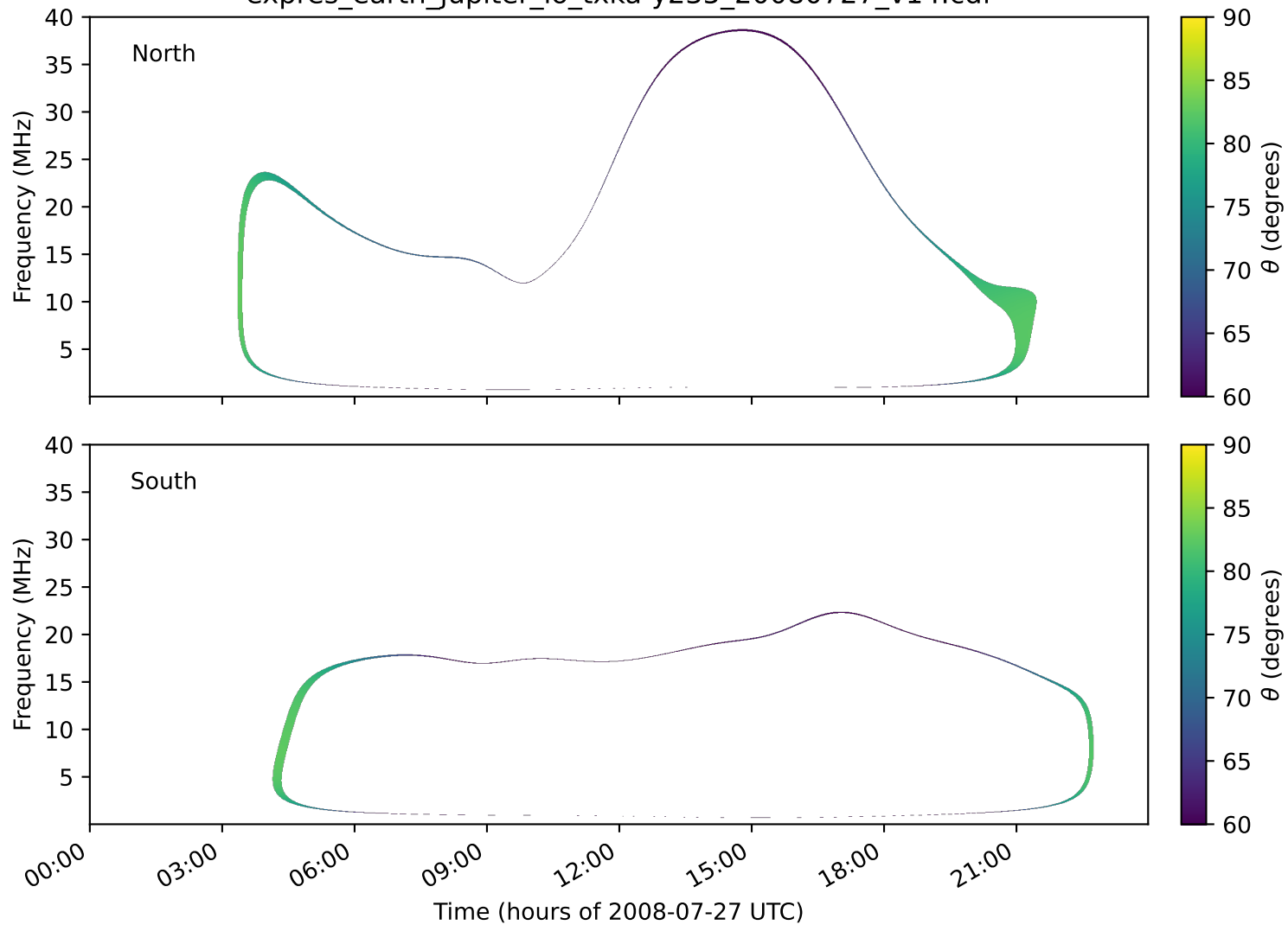
expres_earth_jupiter_io_txka-y235_20080727_v14.cdf
