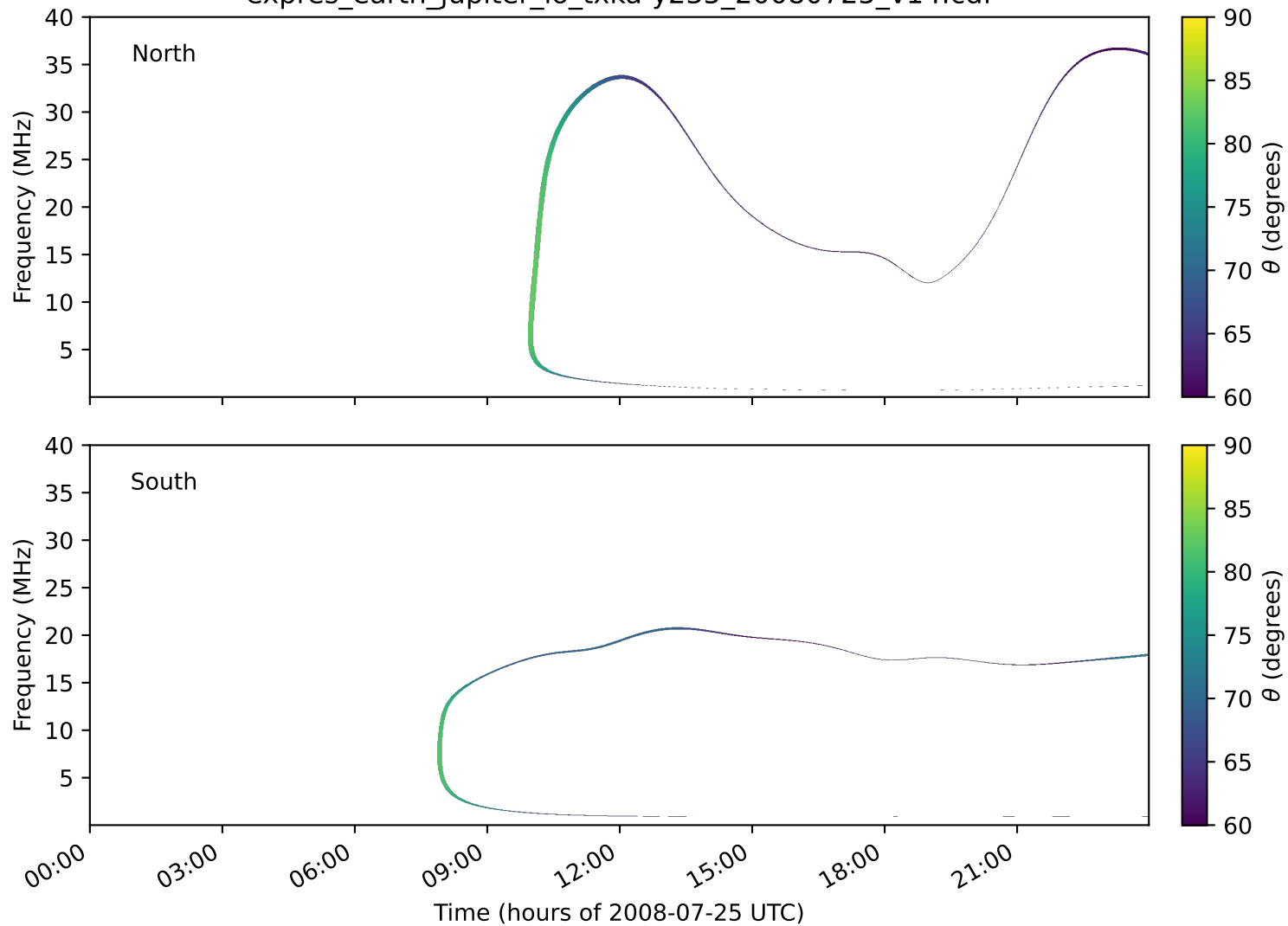
expres_earth_jupiter_io_txka-y235_20080725_v14.cdf
