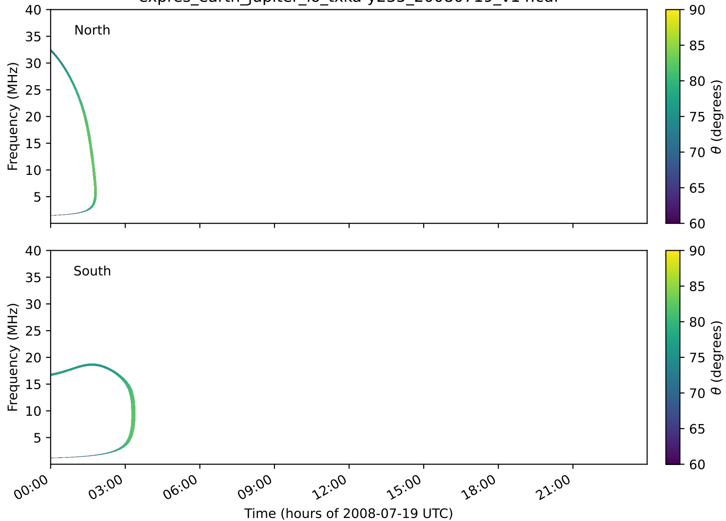
expres_earth_jupiter_io_txka-y235_20080719_v14.cdf
