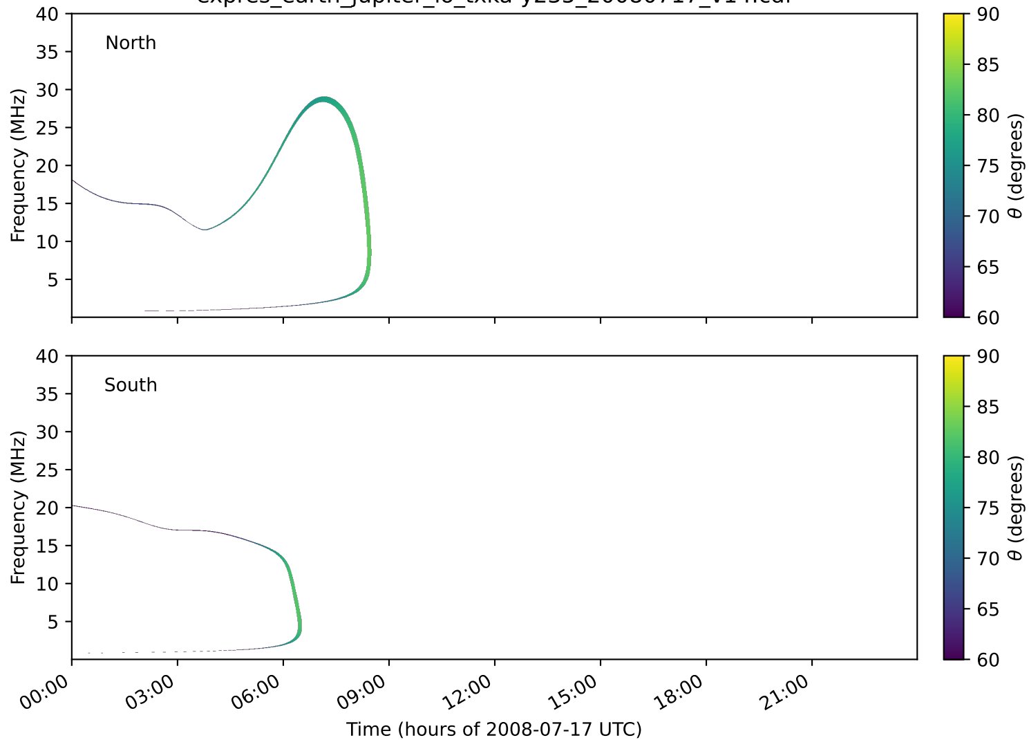
expres_earth_jupiter_io_txka-y235_20080717_v14.cdf
