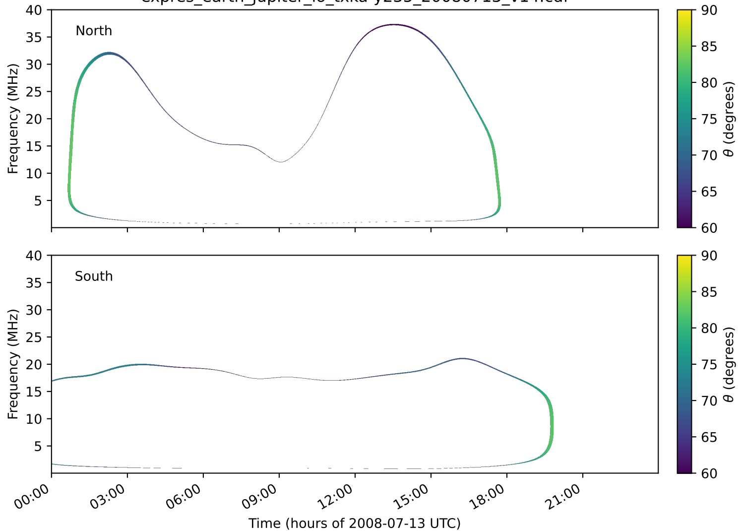
expres_earth_jupiter_io_txka-y235_20080713_v14.cdf
