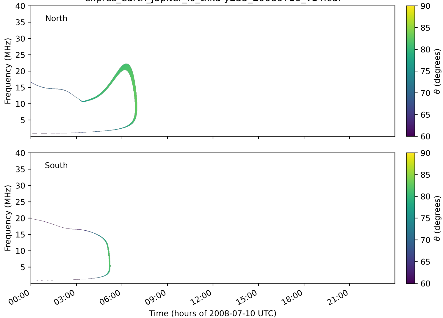
expres_earth_jupiter_io_txka-y235_20080710_v14.cdf
