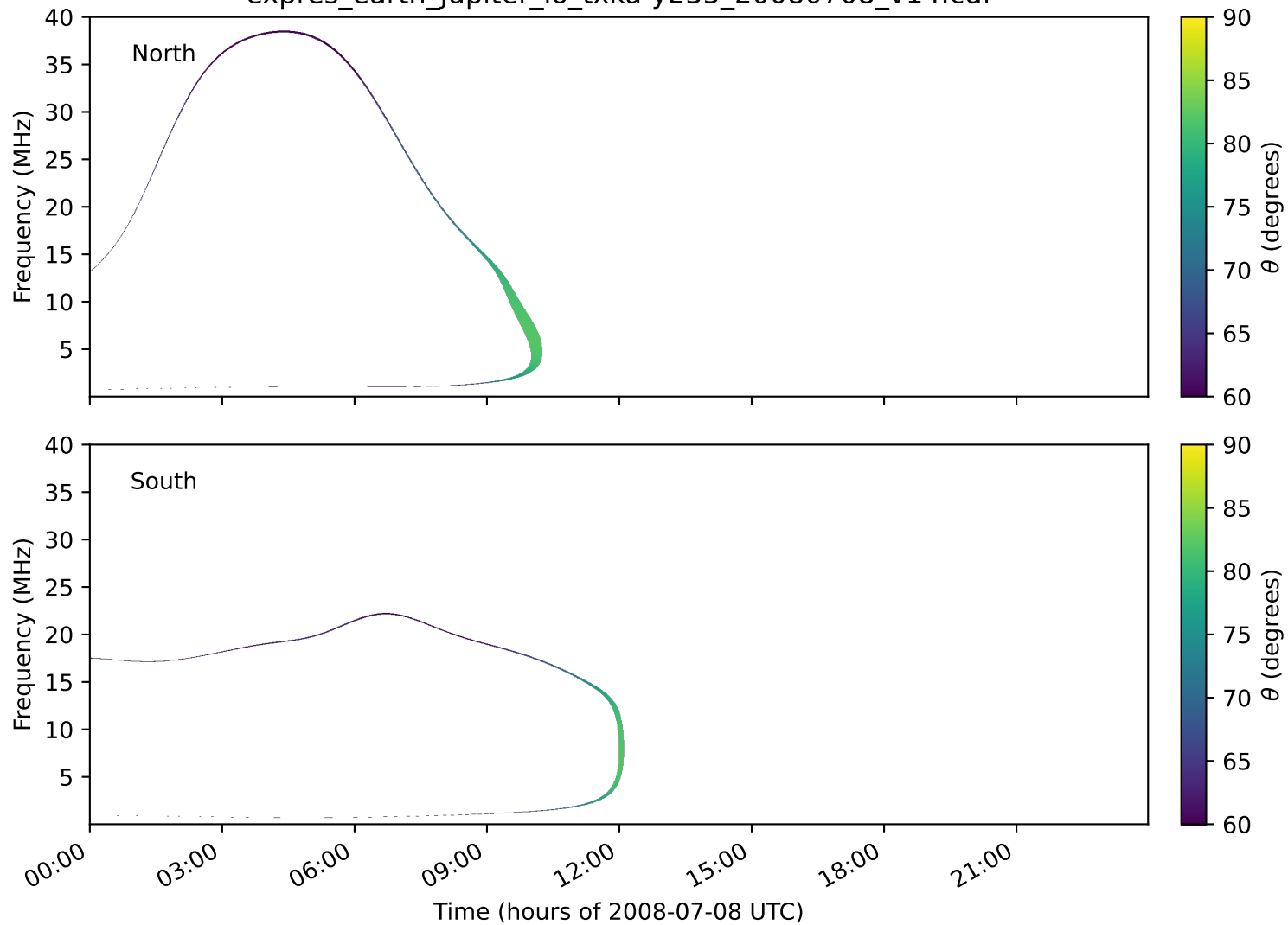
expres_earth_jupiter_io_txka-y235_20080708_v14.cdf
