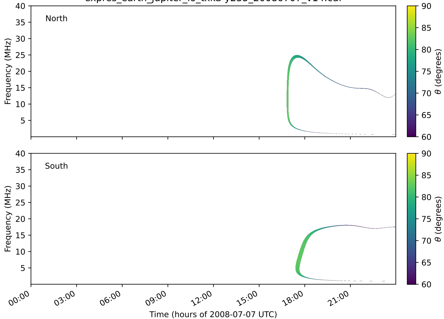
expres_earth_jupiter_io_txka-y235_20080707_v14.cdf
