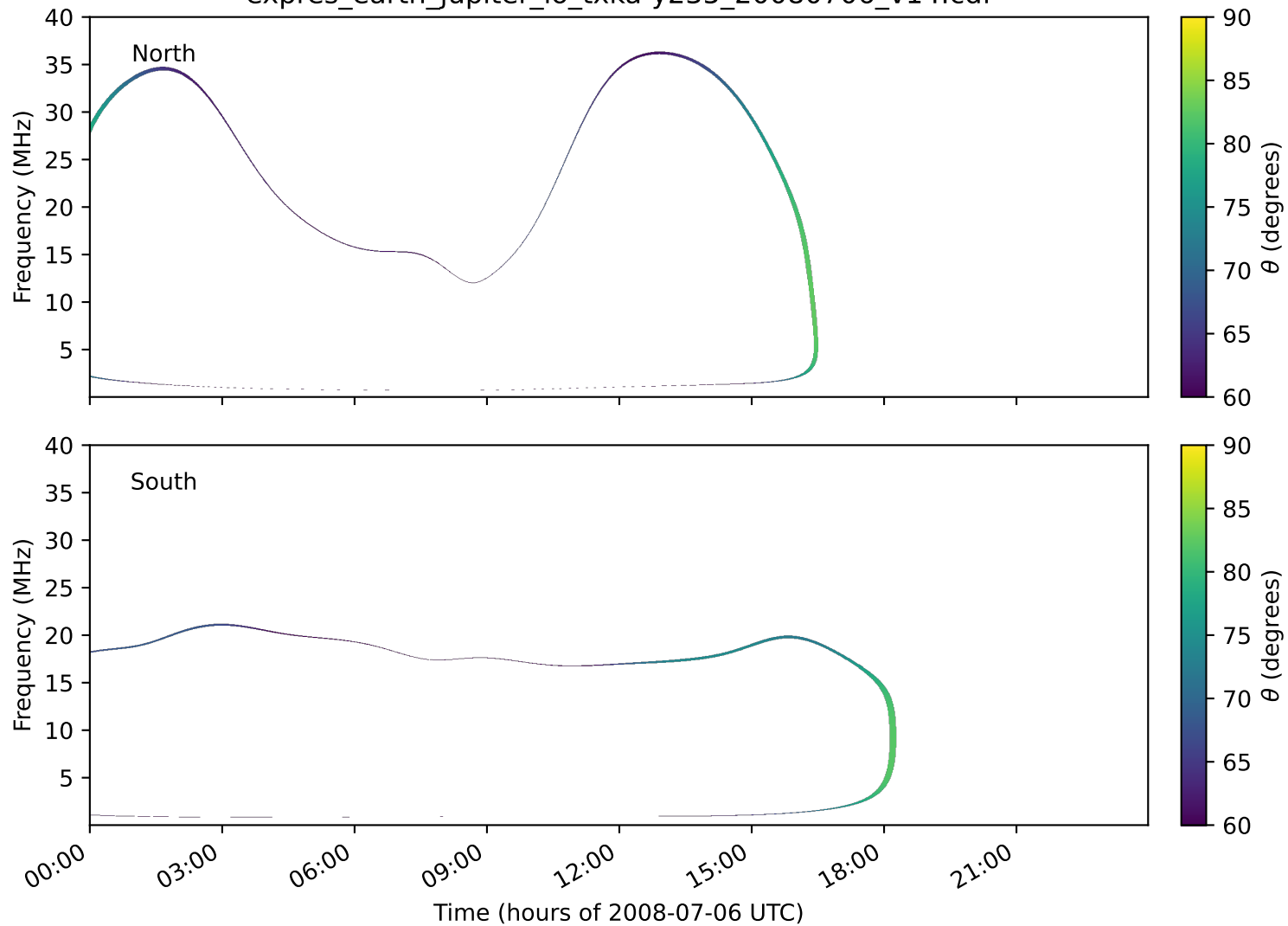
expres_earth_jupiter_io_txka-y235_20080706_v14.cdf
