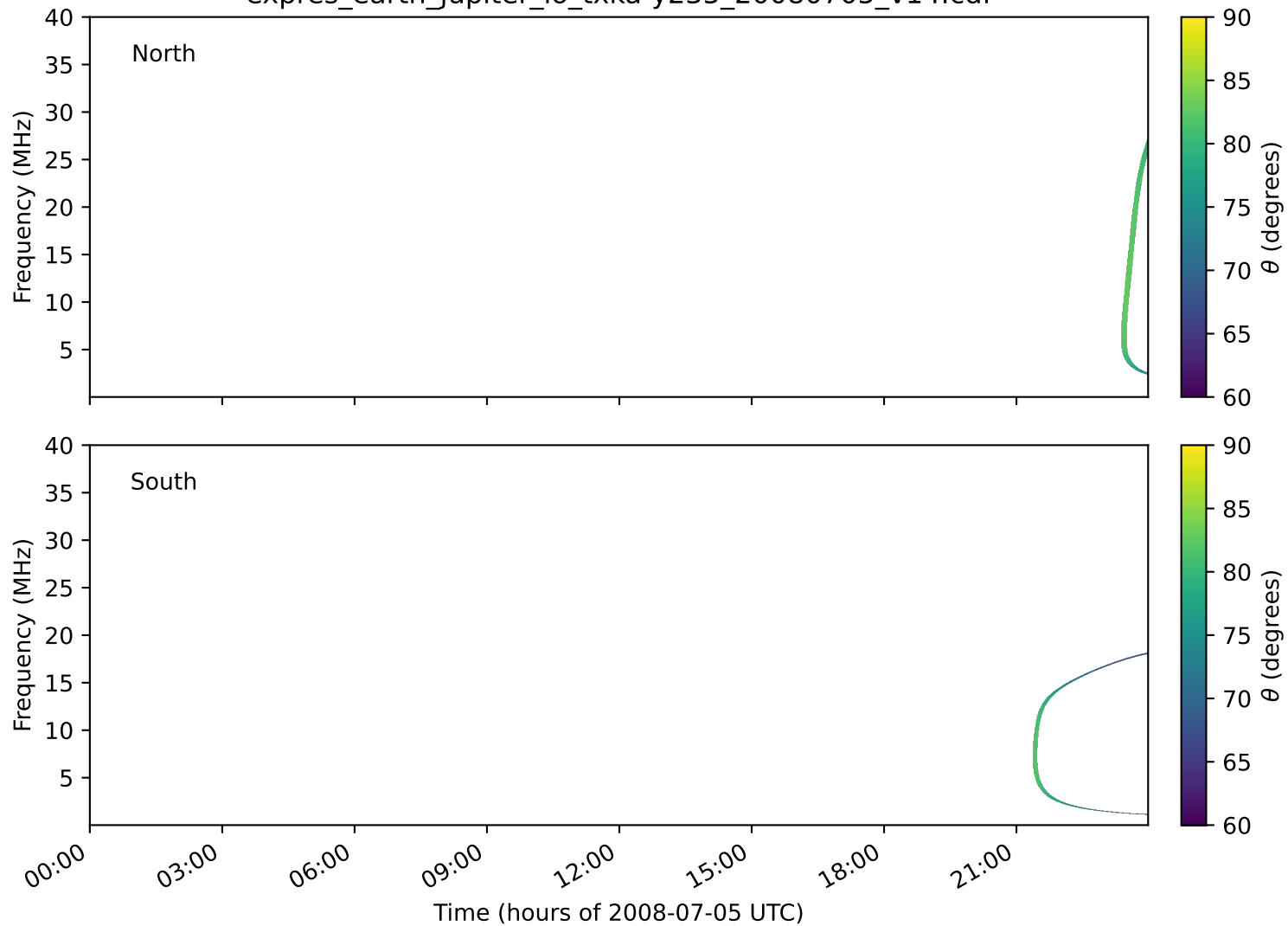
expres_earth_jupiter_io_txka-y235_20080705_v14.cdf
