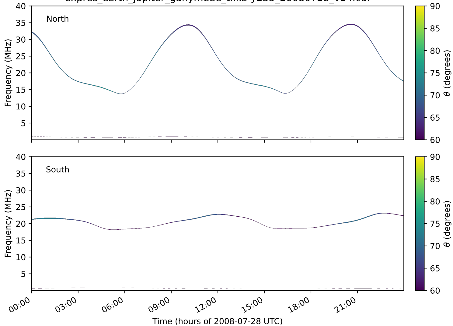
expres_earth_jupiter_ganymede_txka-y235_20080728_v14.cdf
