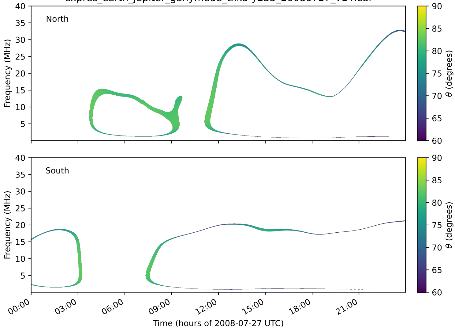
expres_earth_jupiter_ganymede_txka-y235_20080727_v14.cdf
