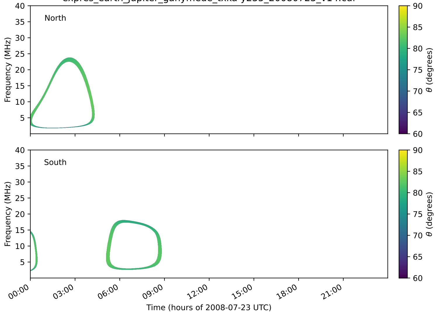
expres_earth_jupiter_ganymede_txka-y235_20080723_v14.cdf
