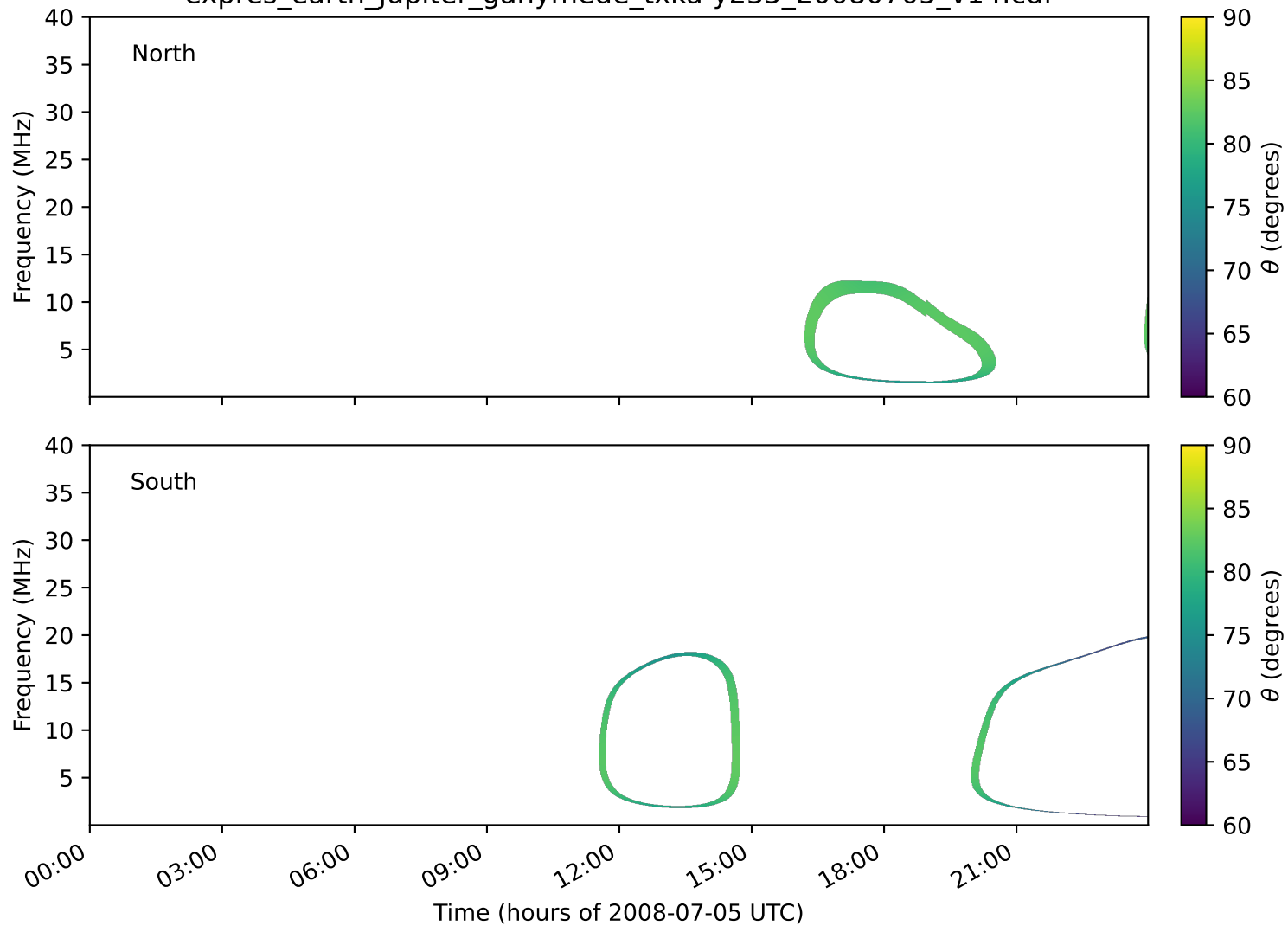
expres_earth_jupiter_ganymede_txka-y235_20080705_v14.cdf
