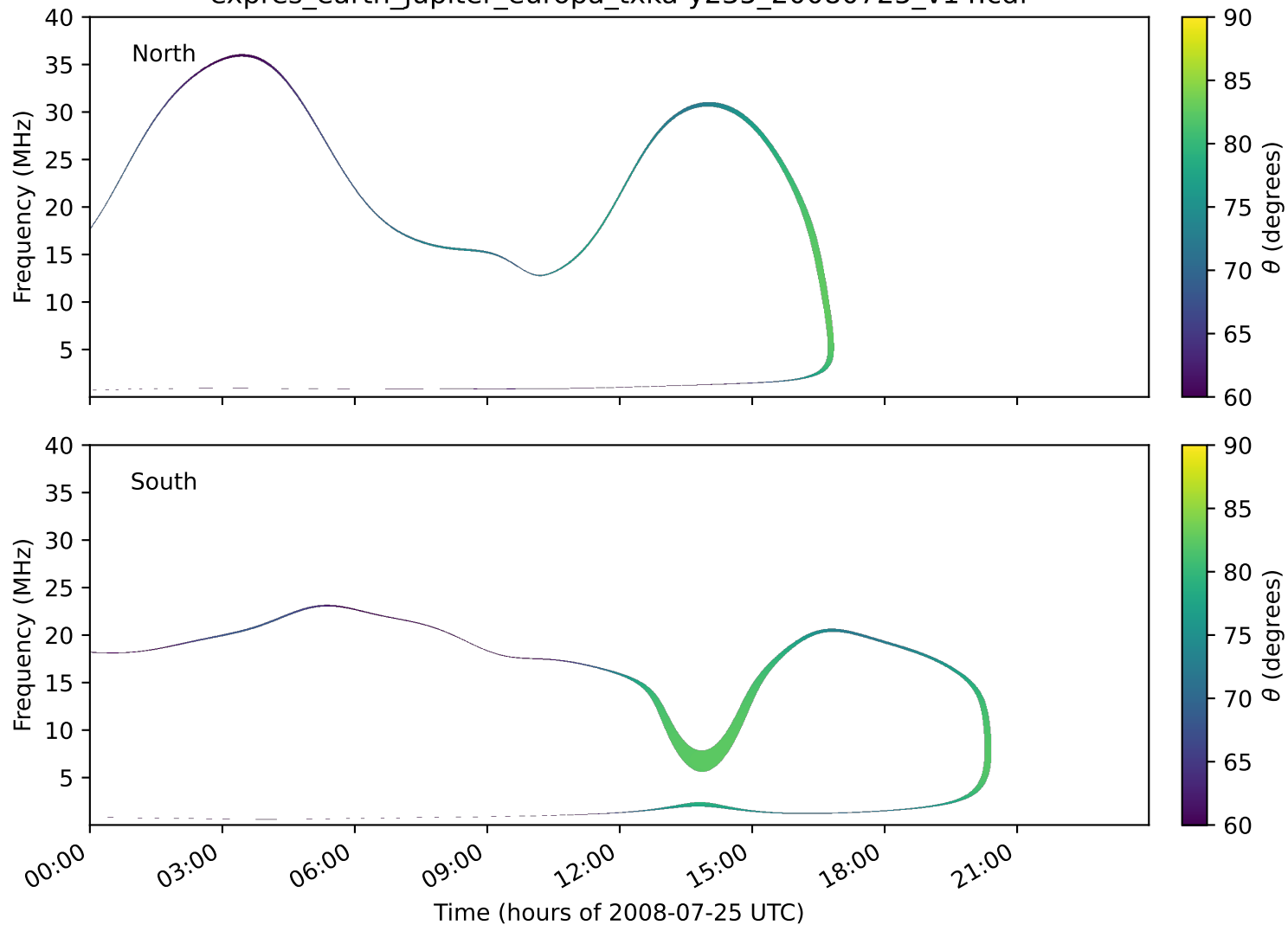
expres_earth_jupiter_europa_txka-y235_20080725_v14.cdf
