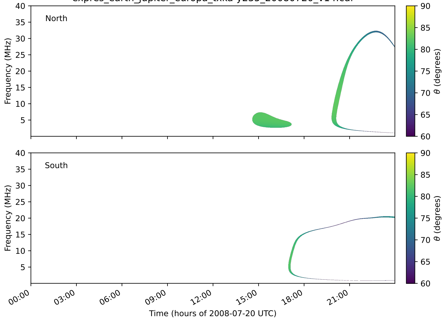
expres_earth_jupiter_europa_txka-y235_20080720_v14.cdf
