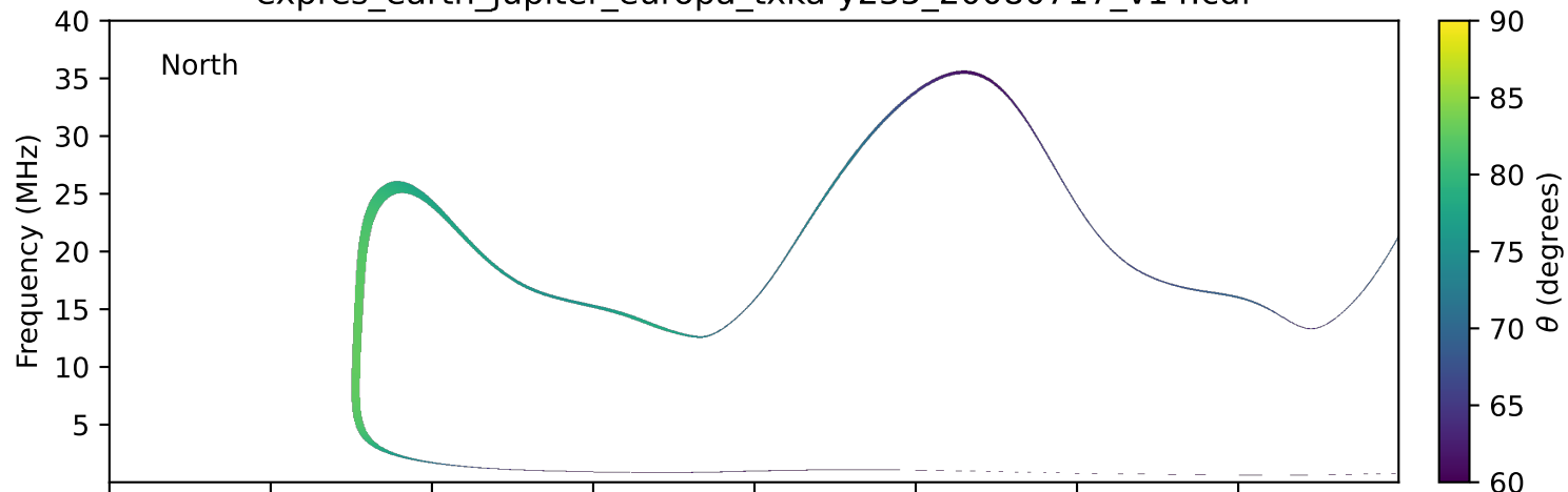
expres_earth_jupiter_europa_txka-y235_20080717_v14.cdf
