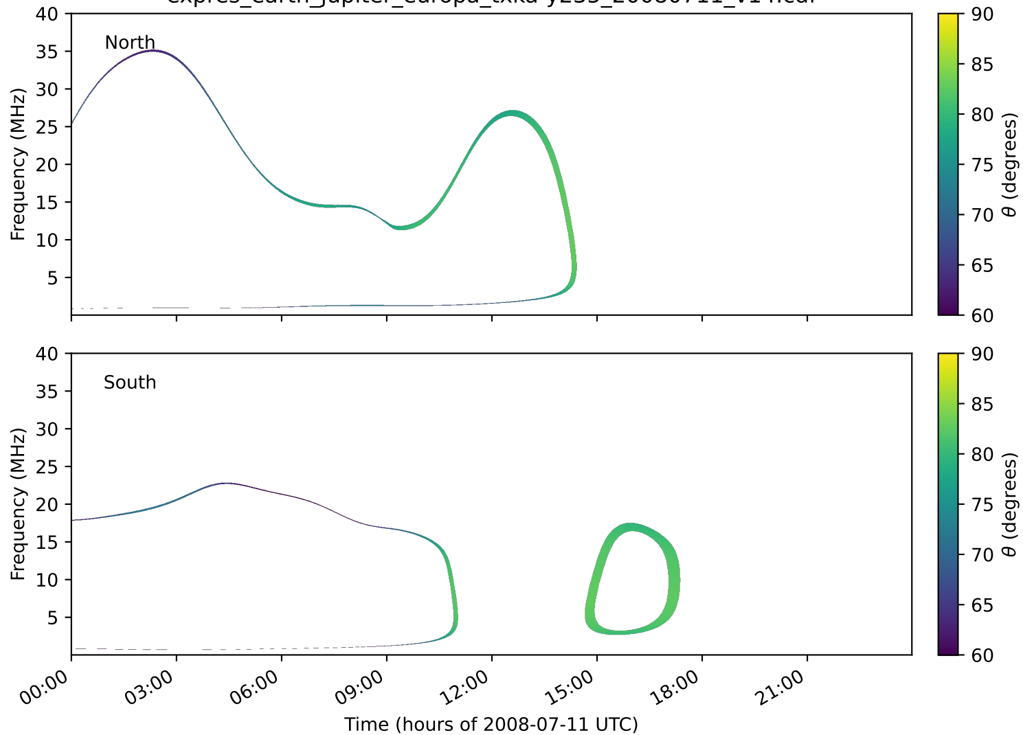
expres_earth_jupiter_europa_txka-y235_20080711_v14.cdf
