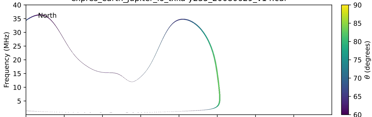
expres_earth_jupiter_io_txka-y235_20080629_v14.cdf
