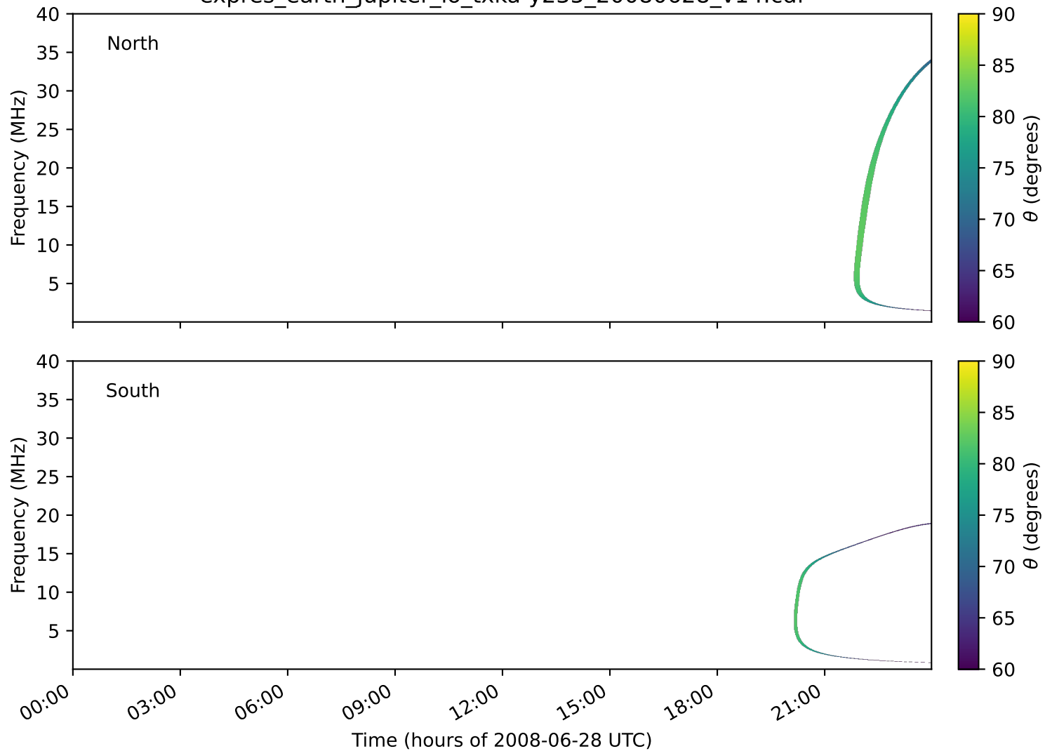
expres_earth_jupiter_io_txka-y235_20080628_v14.cdf
