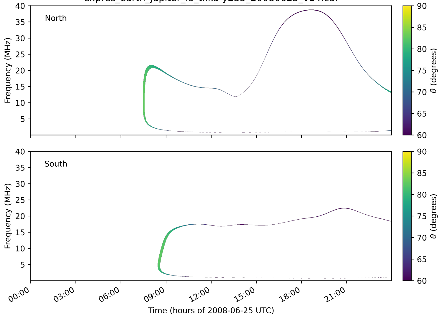
expres_earth_jupiter_io_txka-y235_20080625_v14.cdf
