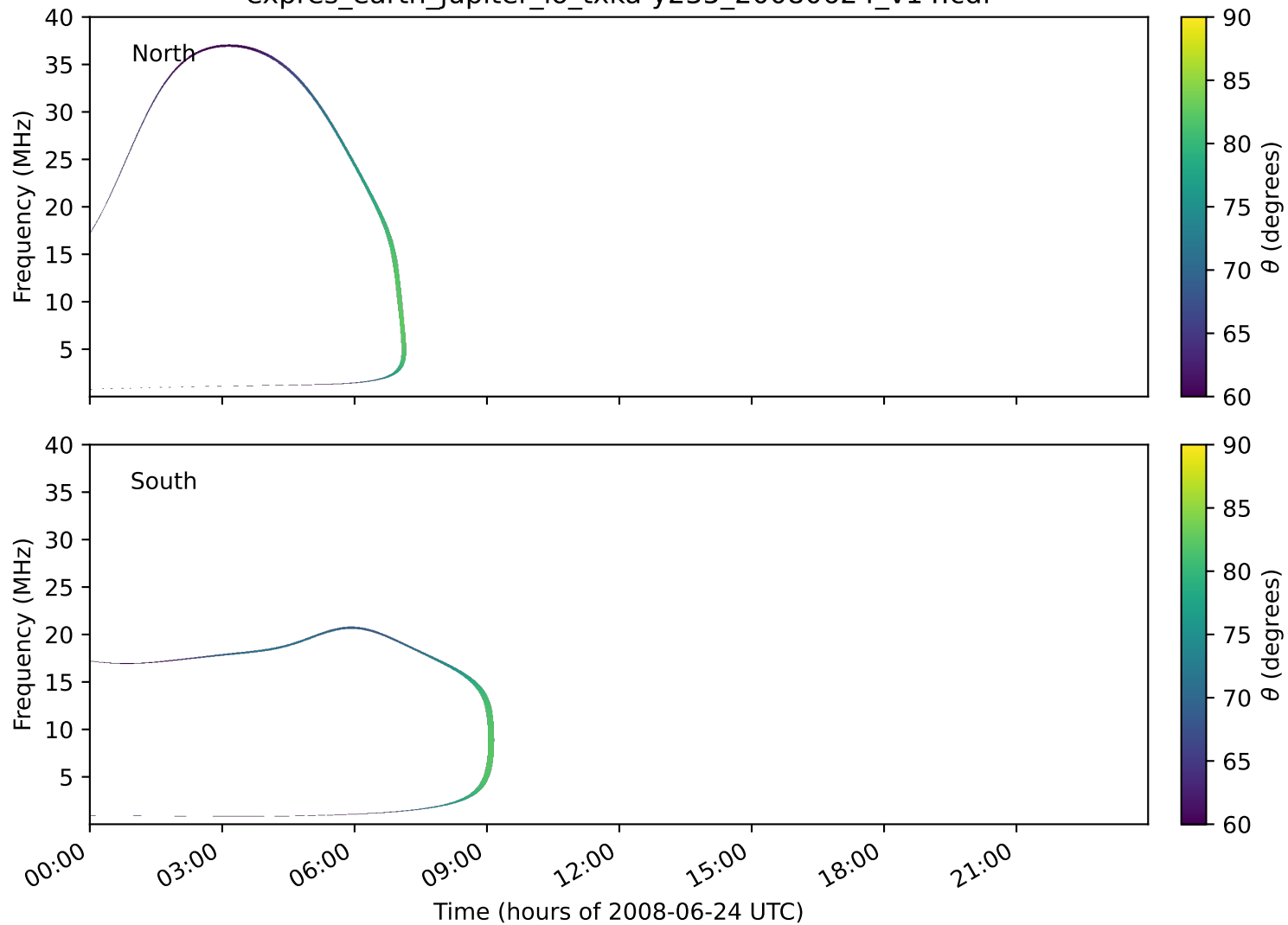
expres_earth_jupiter_io_txka-y235_20080624_v14.cdf
