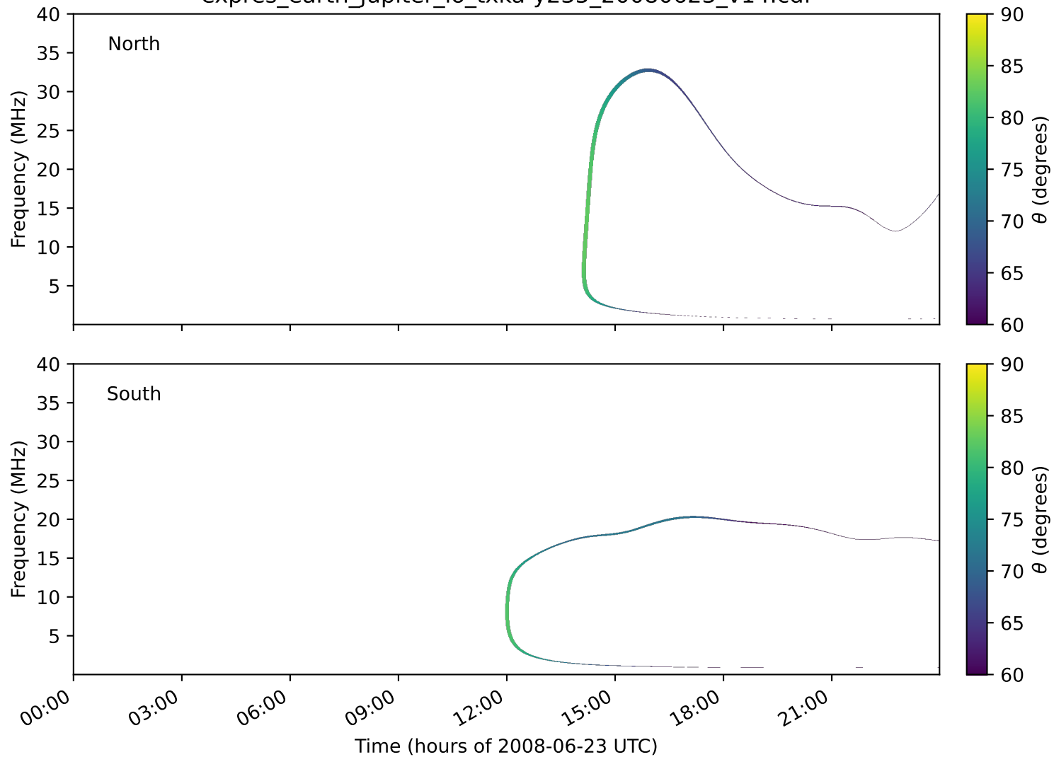
expres_earth_jupiter_io_txka-y235_20080623_v14.cdf
