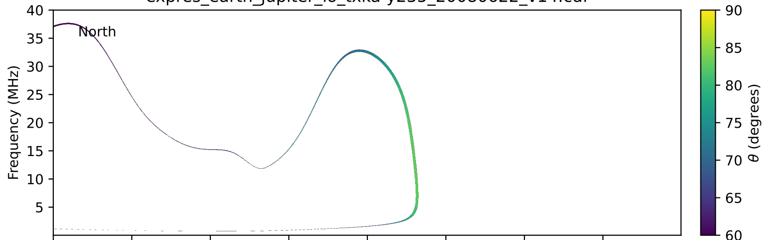
expres_earth_jupiter_io_txka-y235_20080622_v14.cdf
