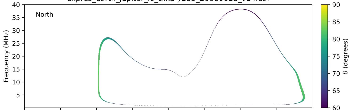
expres_earth_jupiter_io_txka-y235_20080618_v14.cdf
