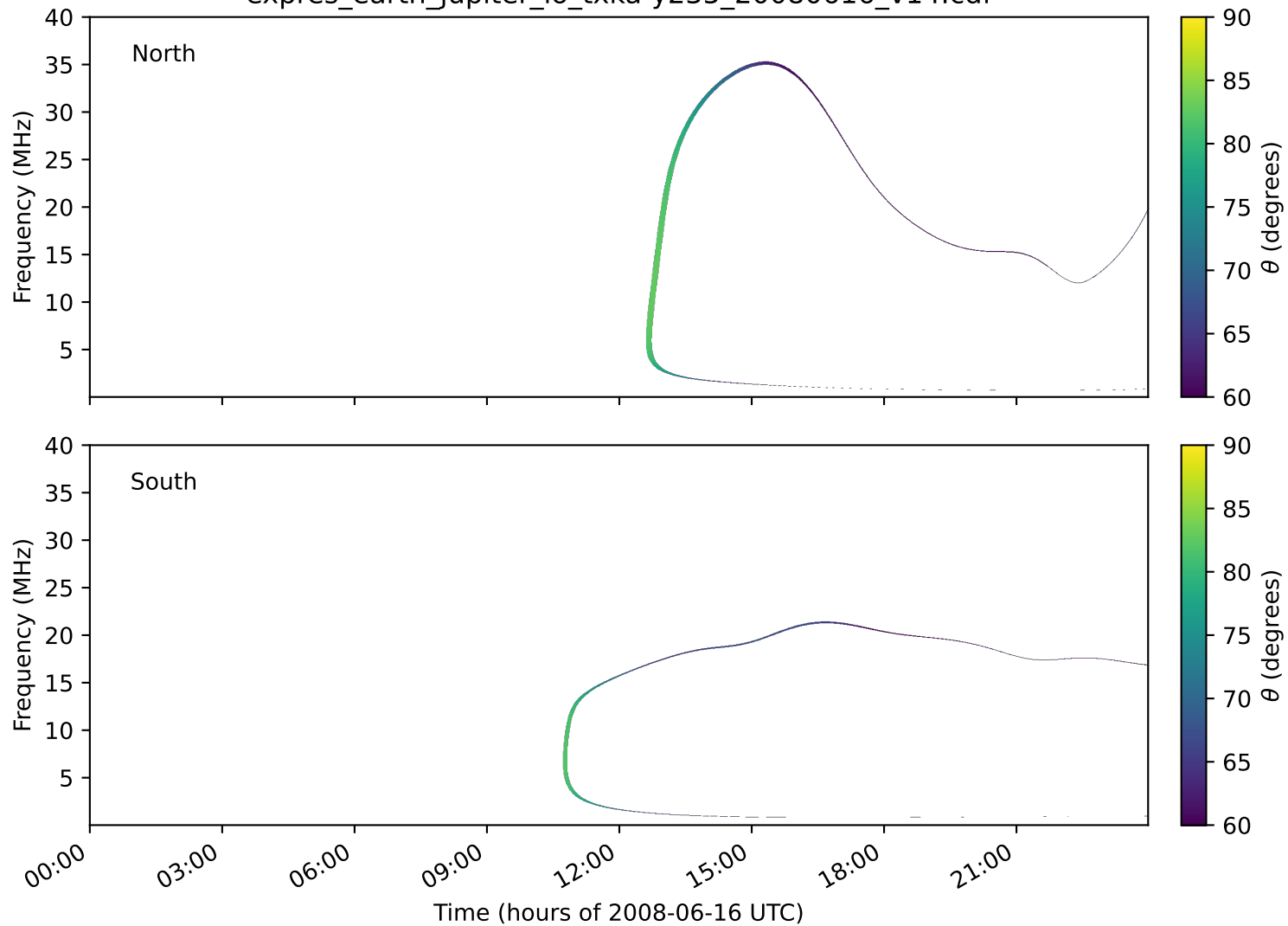
expres_earth_jupiter_io_txka-y235_20080616_v14.cdf
