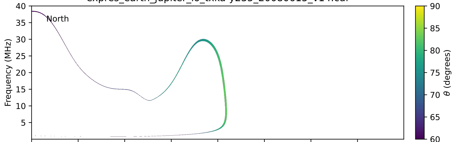
expres_earth_jupiter_io_txka-y235_20080615_v14.cdf
