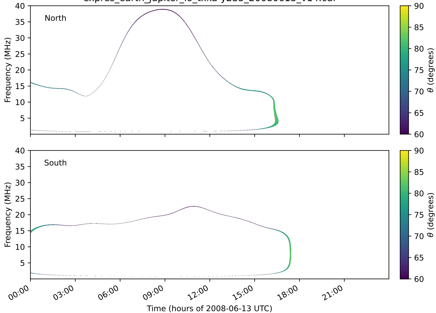
expres_earth_jupiter_io_txka-y235_20080613_v14.cdf
