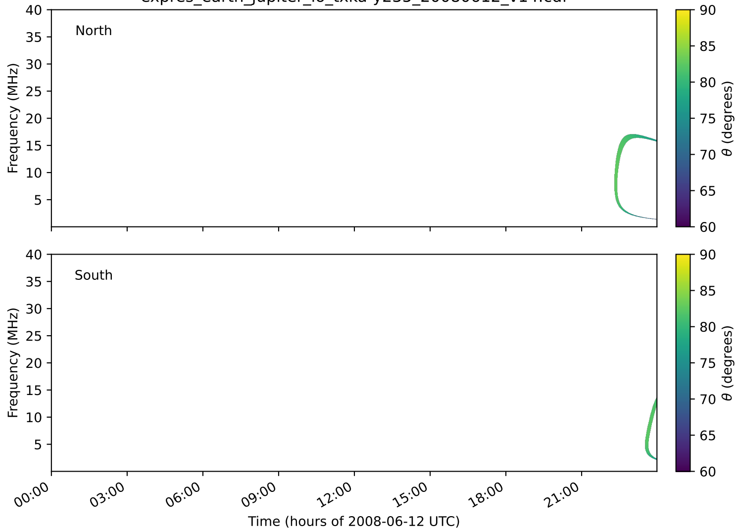
expres_earth_jupiter_io_txka-y235_20080612_v14.cdf
