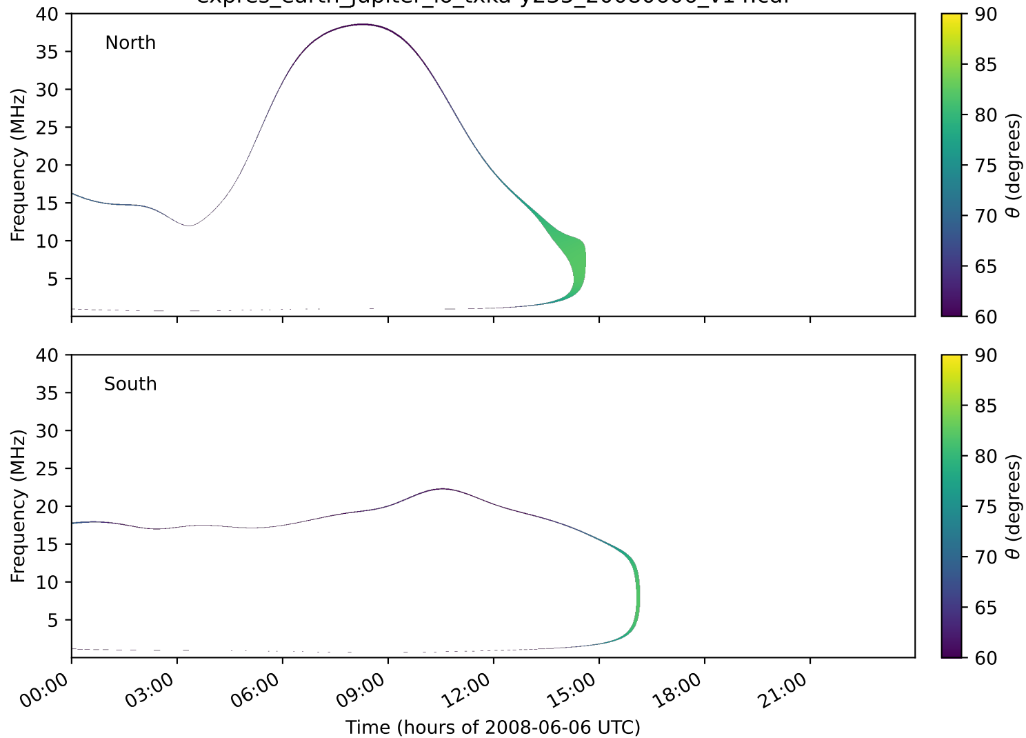
expres_earth_jupiter_io_txka-y235_20080606_v14.cdf
