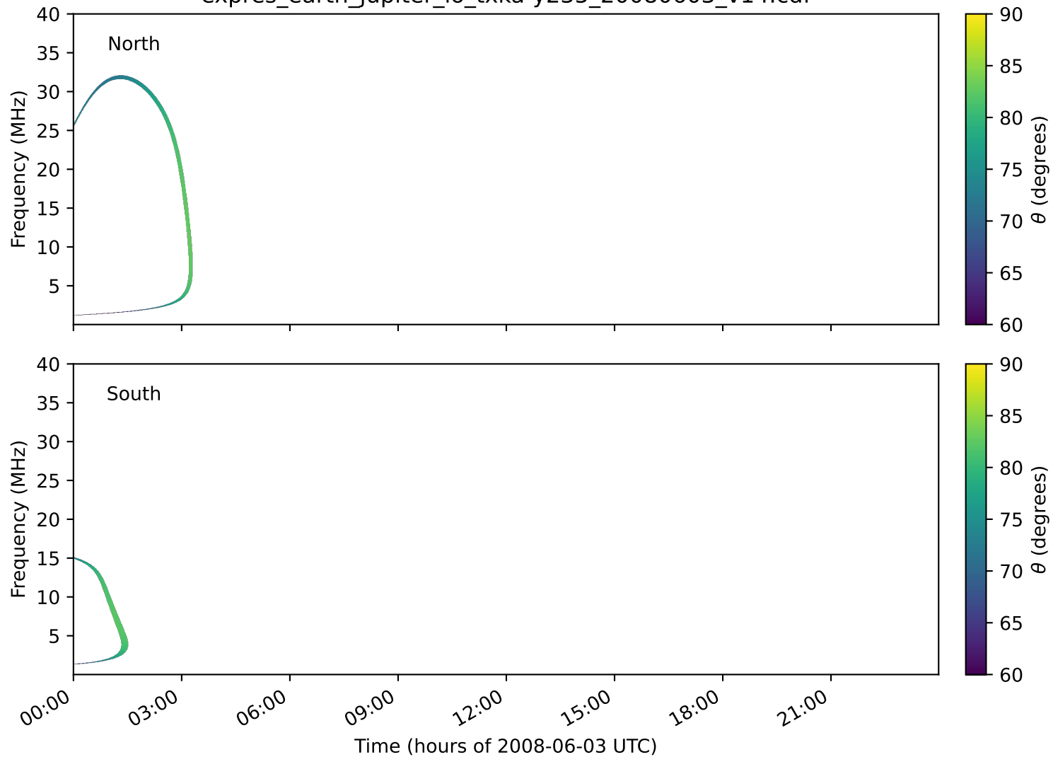
expres_earth_jupiter_io_txka-y235_20080603_v14.cdf
