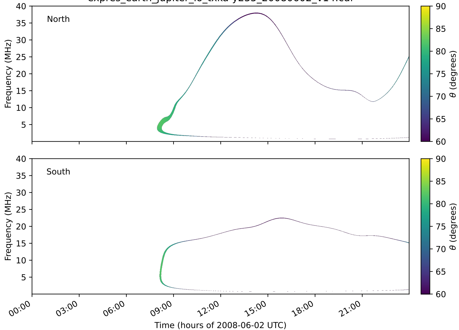
expres_earth_jupiter_io_txka-y235_20080602_v14.cdf
