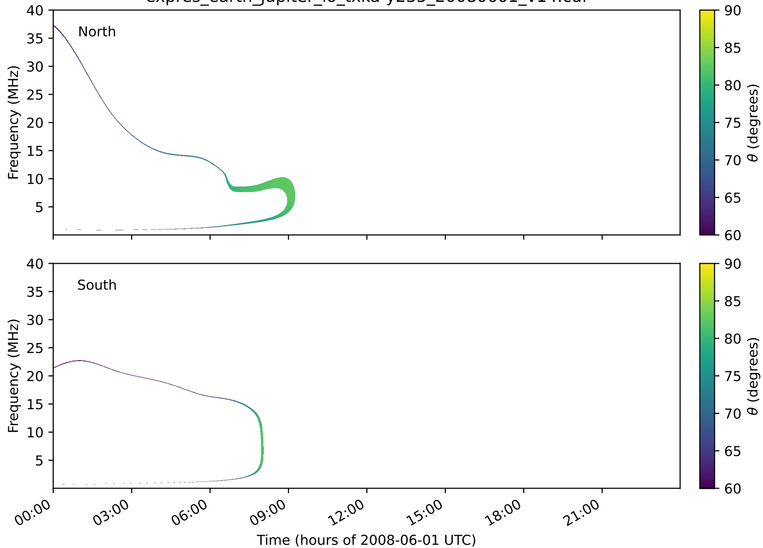
expres_earth_jupiter_io_txka-y235_20080601_v14.cdf
