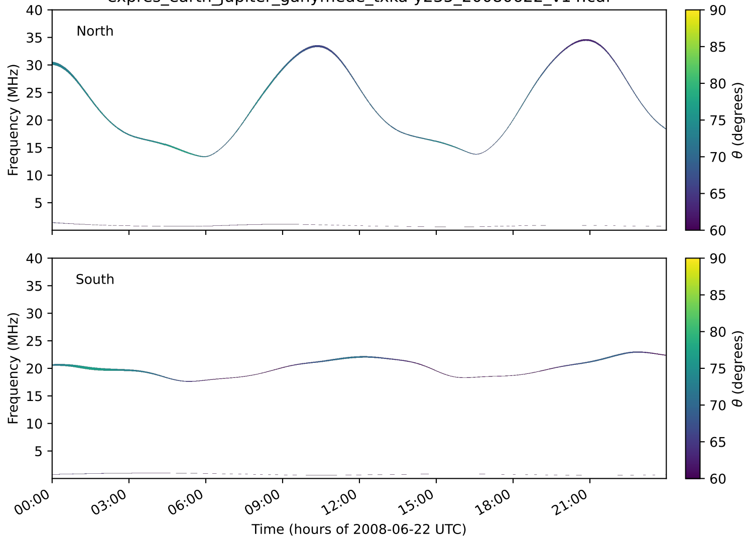
expres_earth_jupiter_ganymede_txka-y235_20080622_v14.cdf
