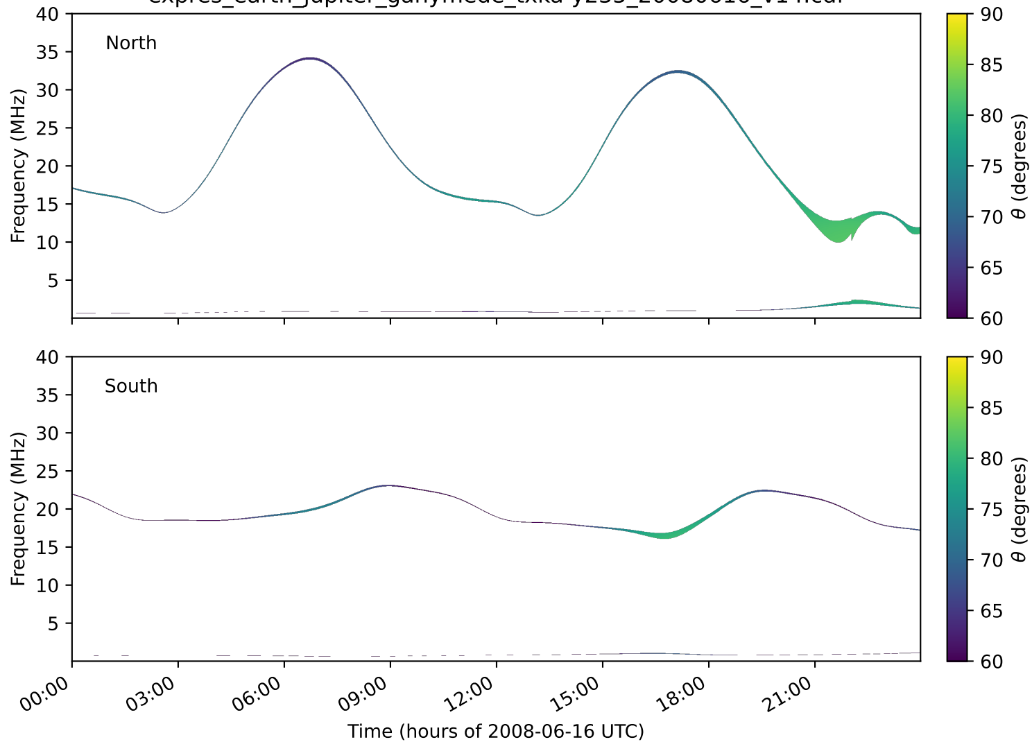
expres_earth_jupiter_ganymede_txka-y235_20080616_v14.cdf
